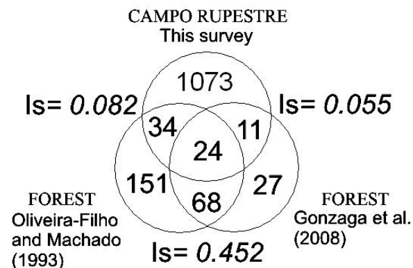
Figure 7. Comparison of the floristic surveys of the Serra de São José campo rupestre (top) and forest checklists by Oliveira-Filho and Machado (1993) and Gonzaga et al. (2008). Numbers represent species or varieties. Is = Sørensen similarity index.
