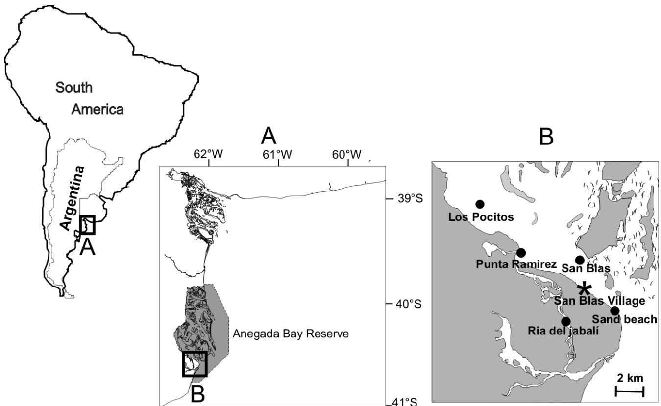
FIGURE 1. Geographic location of study area (A), and sampling sites (B).
