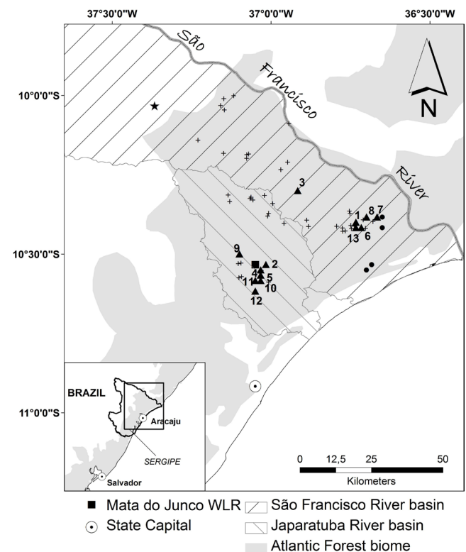
FIGURE 1. Map of the São Francisco and Japarutuba basins in eastern Sergipe, showing the sites surveyed during the present study (▲ = Callicebus coimbrai recorded; + = C. coimbrai not found), localities at which C. coimbrai (●) was recorded in previous studies (Kobayashi and Langguth, 1999; Sousa 2003; Jerusalinsky et al. 2006) and the nearest site at which Callicebus barbarabrownae was recorded in the São Francisco basin (★) by Marques et al. (2013). The sites are numbered as in Table 1.
