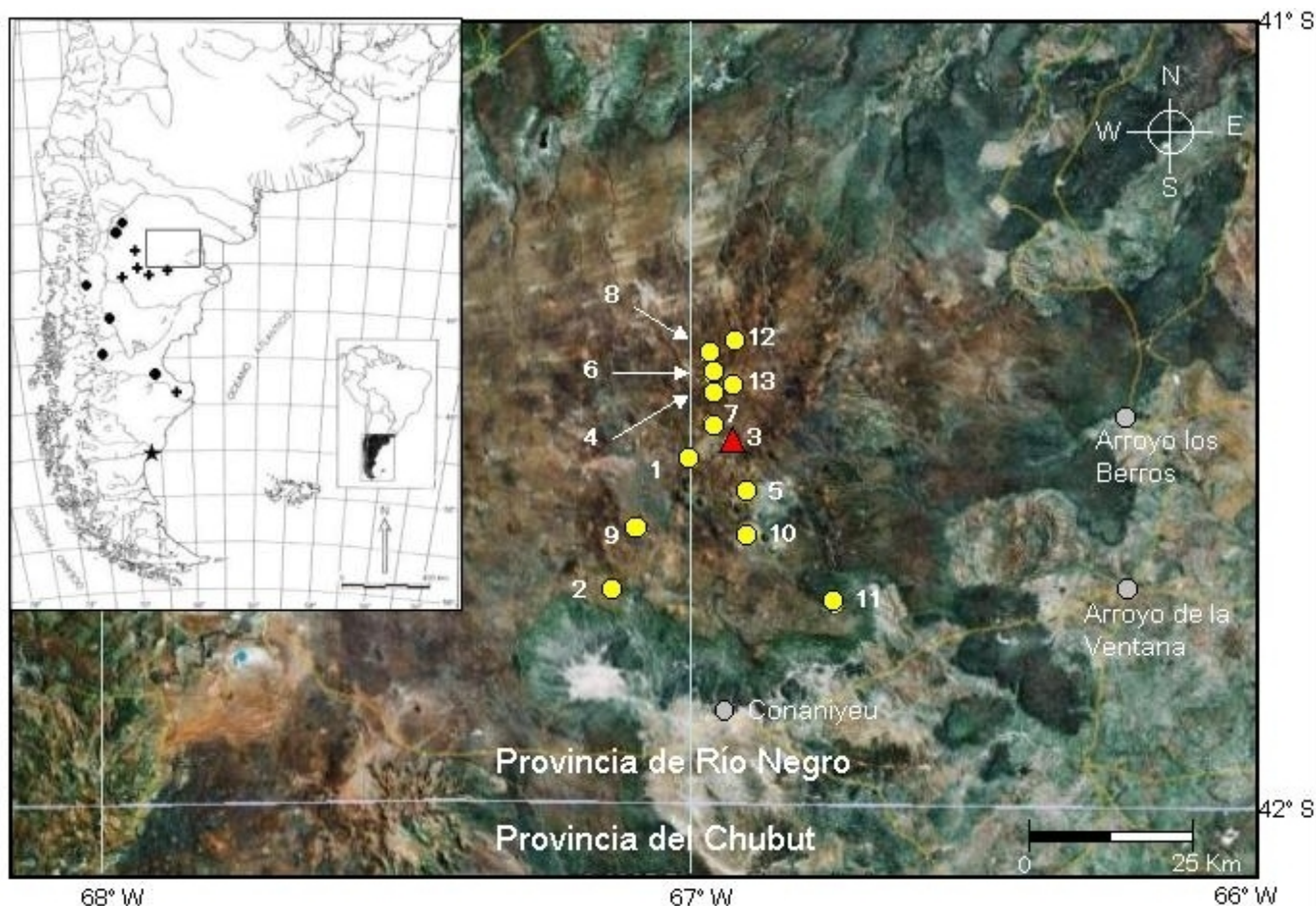
Figure 1. Geographic distribution of Notiomys edwardsii in Patagonia, Argentina. Left: localities reported in literature; star, type locality of Notiomys edwardsii ; circles, animal capture localities; crosses, owl pellets aggregations. Right: Somuncurá plateau; circles represent new localities for Notiomys edwardsii reported here; numbers are detailed in text; triangle is the Corona volcano, the highest elevation of the plateau.
